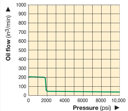
OIL FLOW vs. PRESSURE
