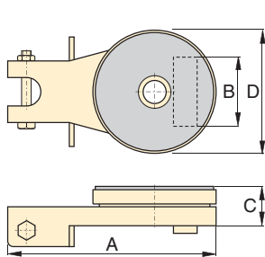
Turntable Swivel ES-1, ES-10, ES-15, ES-30
