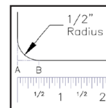
MINIMUM EDGE RADII SUITABLE FOR CONTACT WITH UNPROTECTED WEB SLINGS
