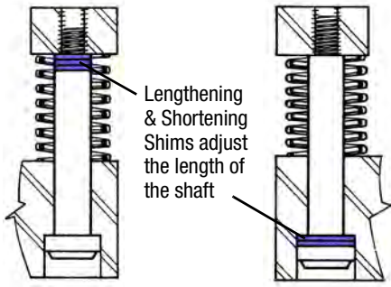
Lengthening Shims
