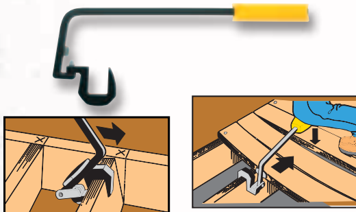
Straighten joists.
